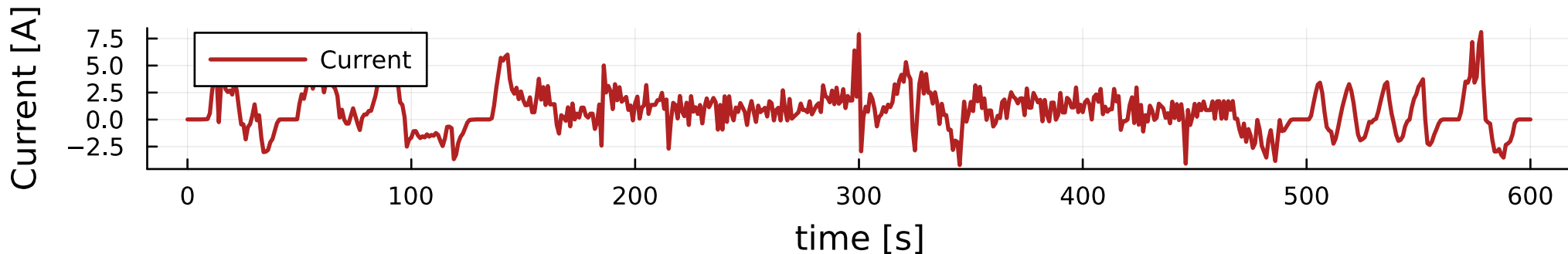
US06 Current Profile
